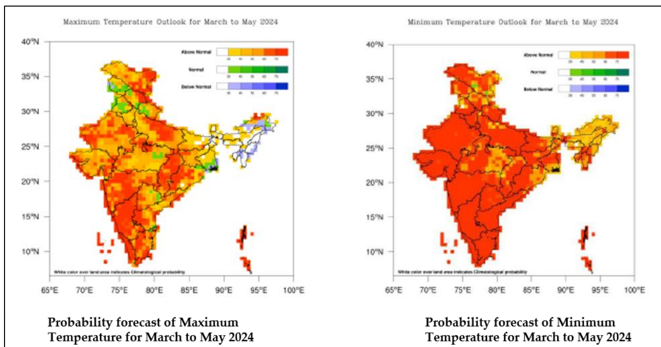
Fig 12a: Probability of Max & Min temperature outlook during March to May (MAM) 2024
