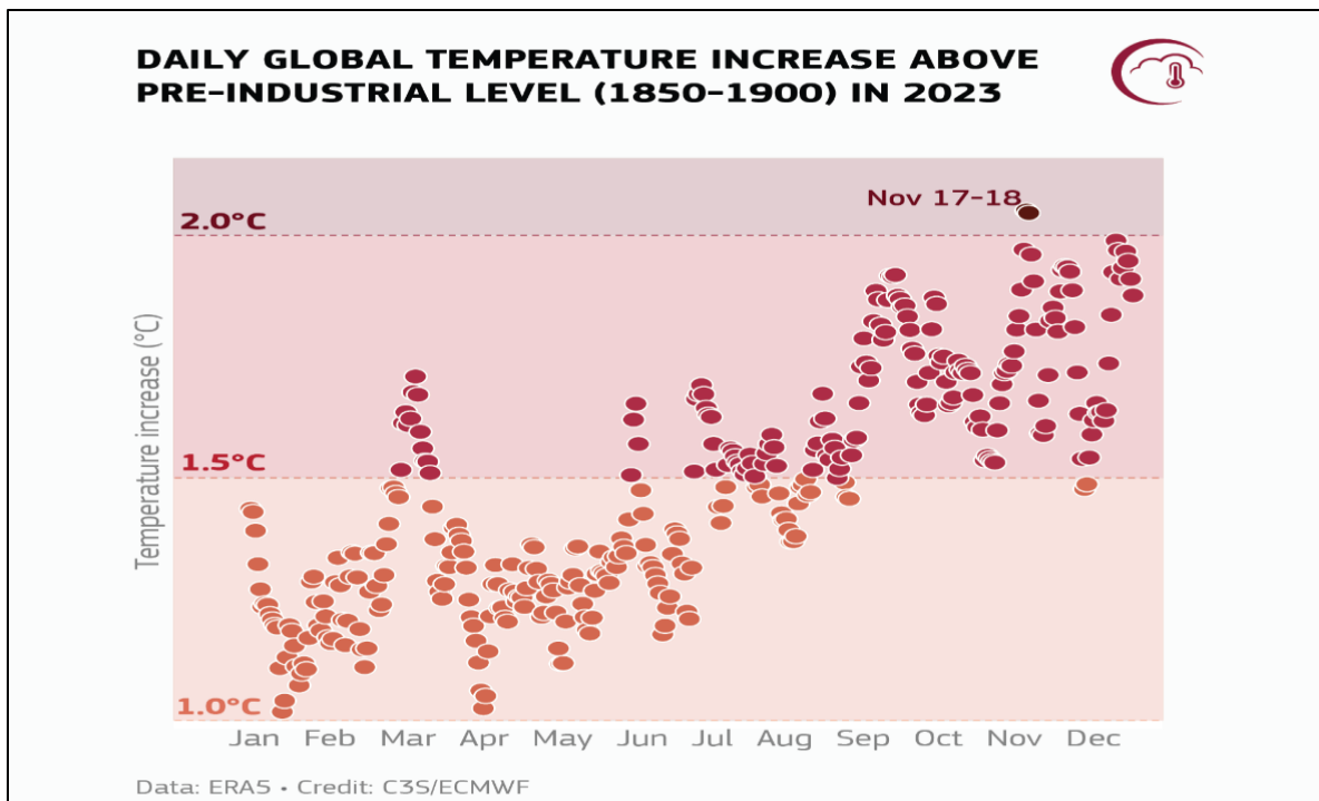
Fig1: Daily global surface air temperatures for 2023, indicating the increase above the average for 1850–1900, the designated pre-industrial reference period. The plot highlights temperature increases within three ranges: 1– 1.5^{\circ}\text{C} (orange), 1.5 – 2^{\circ}\text{C} (red), and above 2^{\circ}\text{C} (crimson). Source: ERA5. (Source: C3S/ECMWF)
