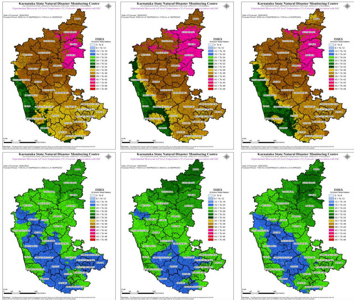
Fig 13: Temperature forecast map at Gram panchayat level for next three days with 12 hours interval as on 18 th April, 2023
